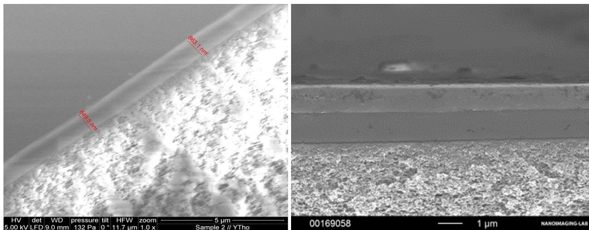
Scanning electron microscopy (SEM) pictures of a polymer thin film and a multilayer membrane from DeltaMem AG
